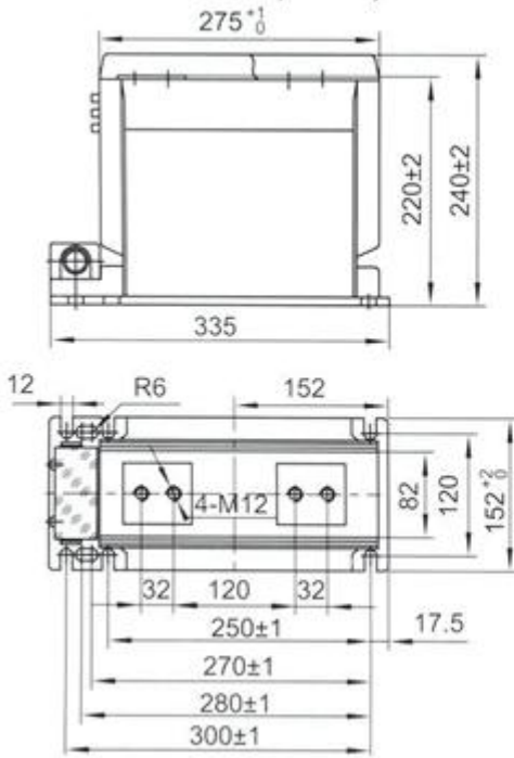
LZZBJ9-12/150b/2s
