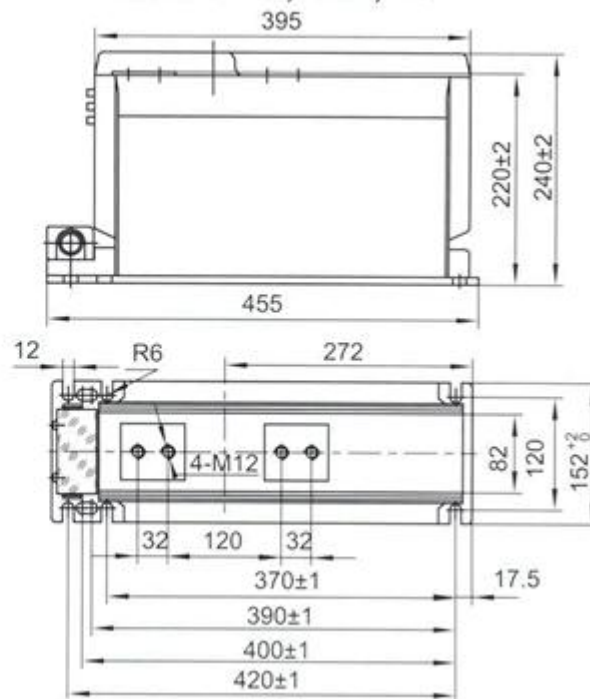
LZZBJ9-12/150b/4s
